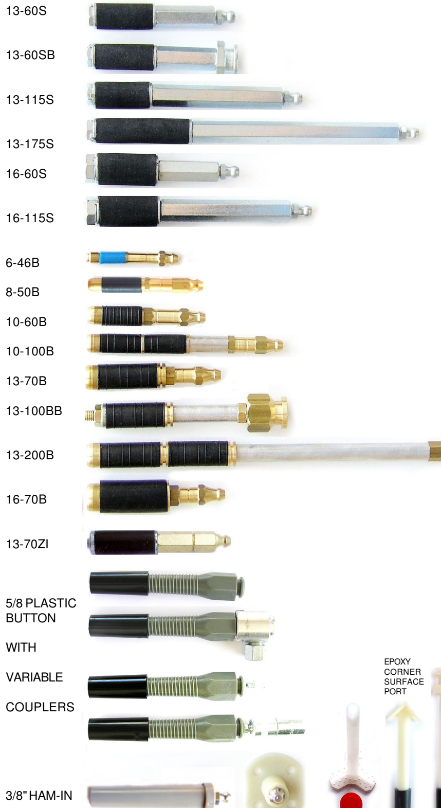
PLASTIC SURFACE PORT WITH ZERK
