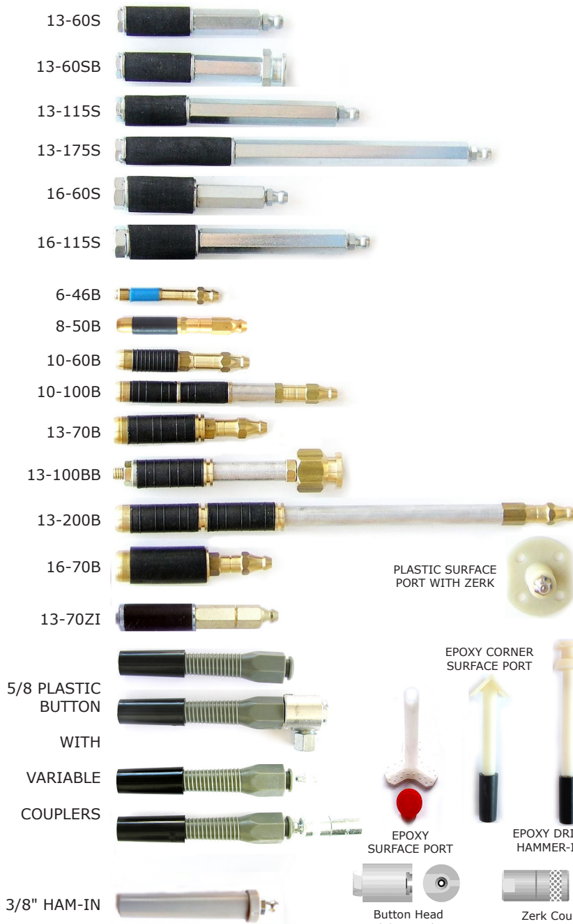
Button Head Slide Coupler
