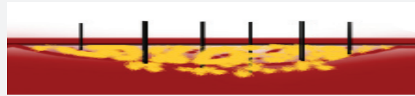
Injecting SealBoss® 1640 SlabLifter Foam through injection needles into soil cavity under roadway
